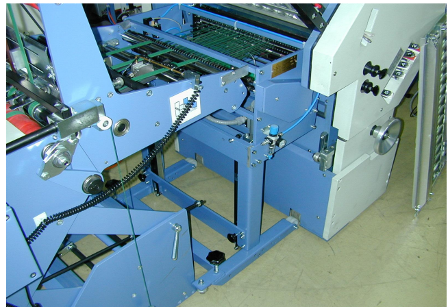
Vertical delivery unit 271 together in use with marking device
