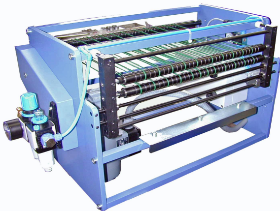
Marking device for use in front of delivery unit
