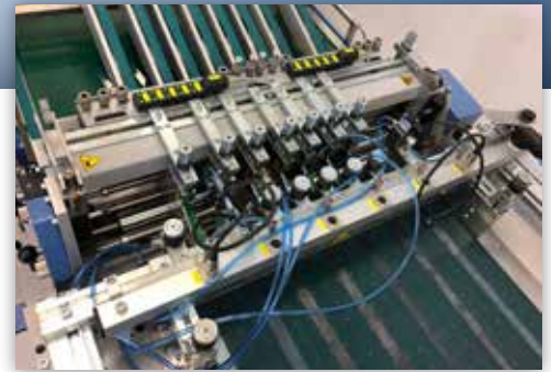
Integral Stripping
